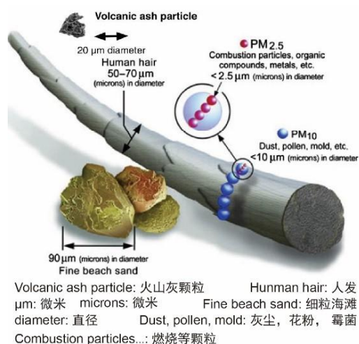
图22. 火山灰形貌和尺寸 (图片来自EOV, Image from the US EPA)
